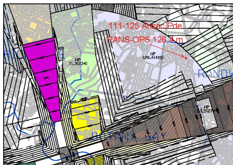
Figure 4.1 PANS-OPS Approach Surfaces
