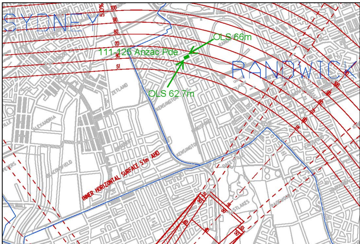
Figure 3.1 - Development site in relation to the OLS surfaces (from Sydney Airport OLS Chart)
